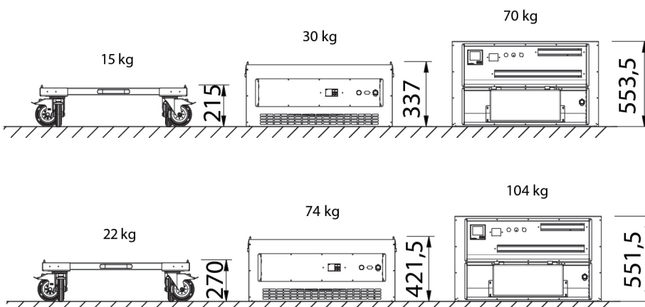
Fig.1 Wärtsilä JOVYLOAD EASY and EASY XL dismounted into 3 parts
